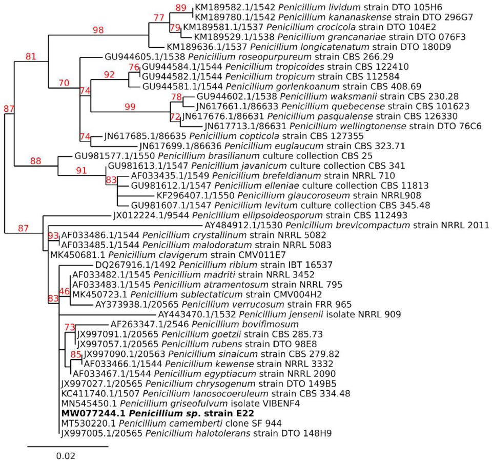
Fig. 1. Phylogenetic tree of ITS region sequences inferred by maximum-likelihood method. Numbers above branches indicate 1000 bootstrap replicates values and 44 sequences of Penicillium species used are presented with GenBank accession numbers followed by the name of strains.
