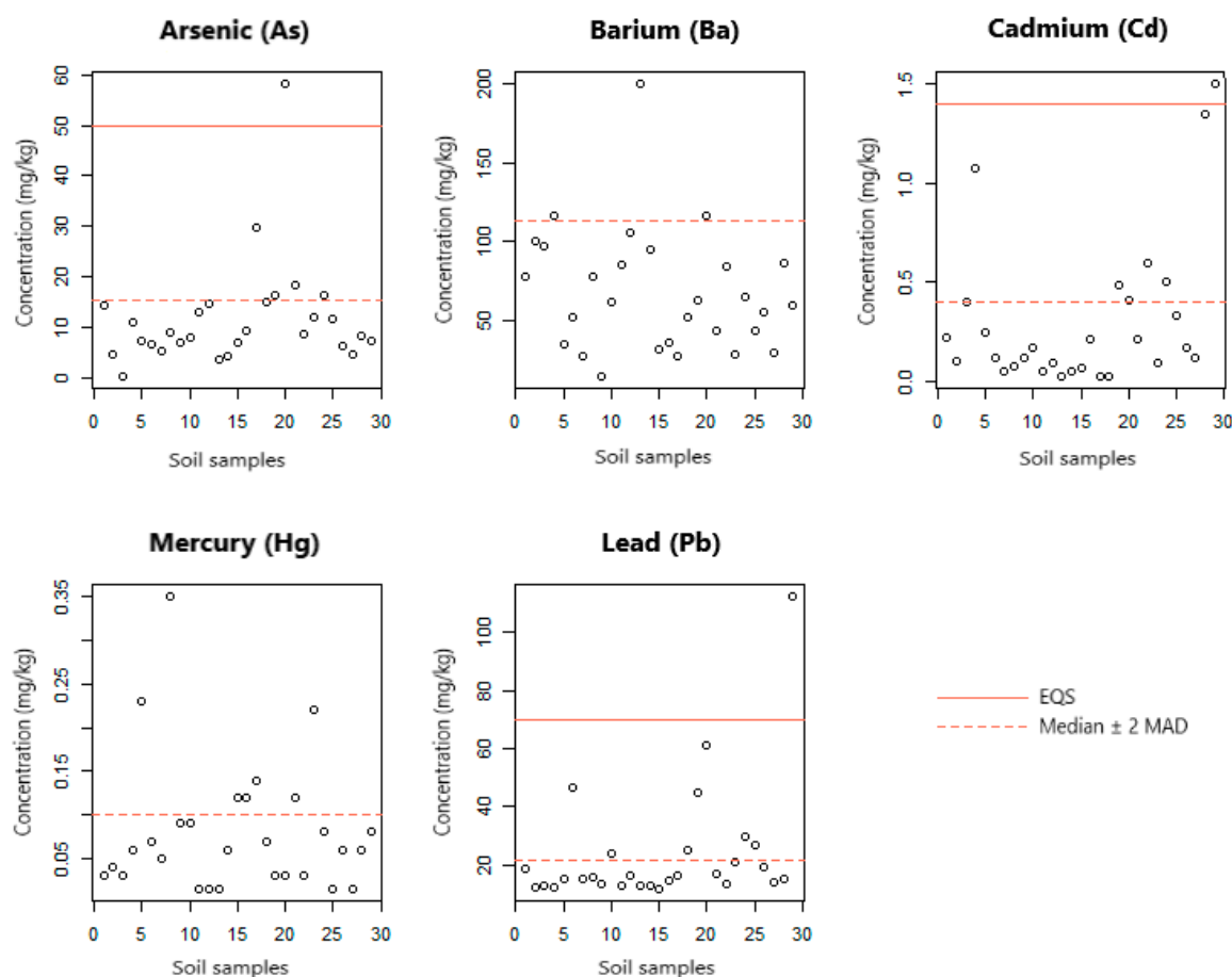
Figure 4. Threshold values and soil sample distribution for As, Ba, Cd, Hg, and Pb with EQS values and geochemical baseline values by median method.
