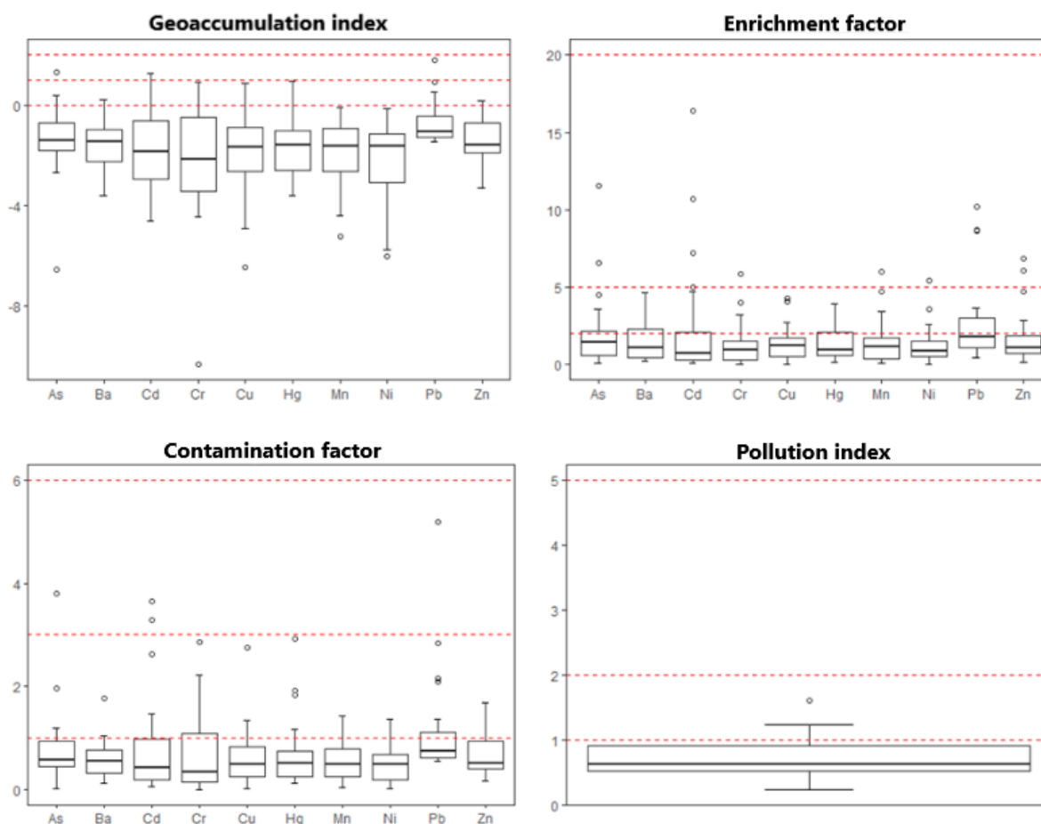
Figure 5. Box-plot diagram for ecological indices using geochemical baseline values using the median \pm 2 MAD method. The red dashed lines point out the classification of each environmental index.
