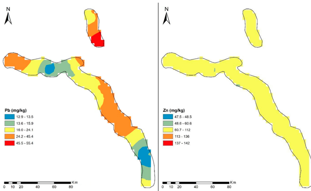
Figure 10. Spatial distribution of Pb and Zn concentrations (mg/kg).
