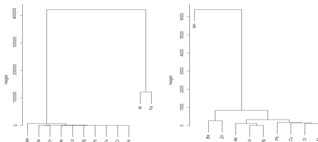
Figure 3. Dendrograms of cluster analysis, using Ward's method, of heavy metals in surface soil (0–25 cm) of the project.
