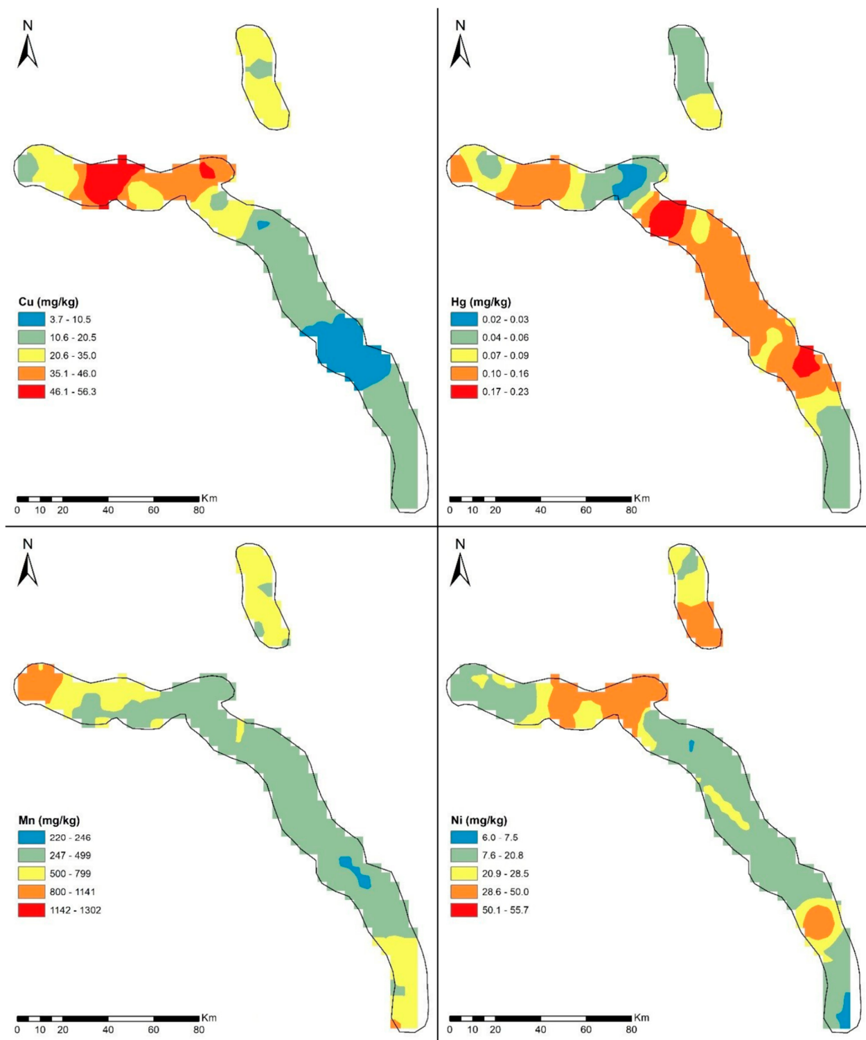
Figure 9. Spatial distribution of Cu, Hg, Mn, and Ni concentrations (mg/kg).
