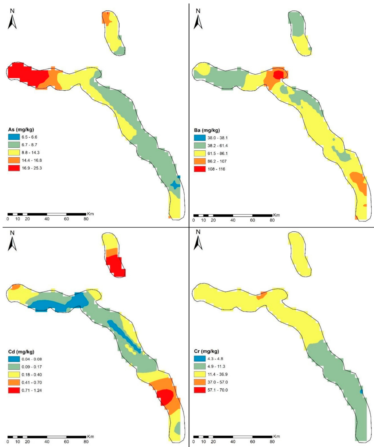
Figure 8. Spatial distribution of As, Ba, Cd, and Cr concentrations (mg/kg).
