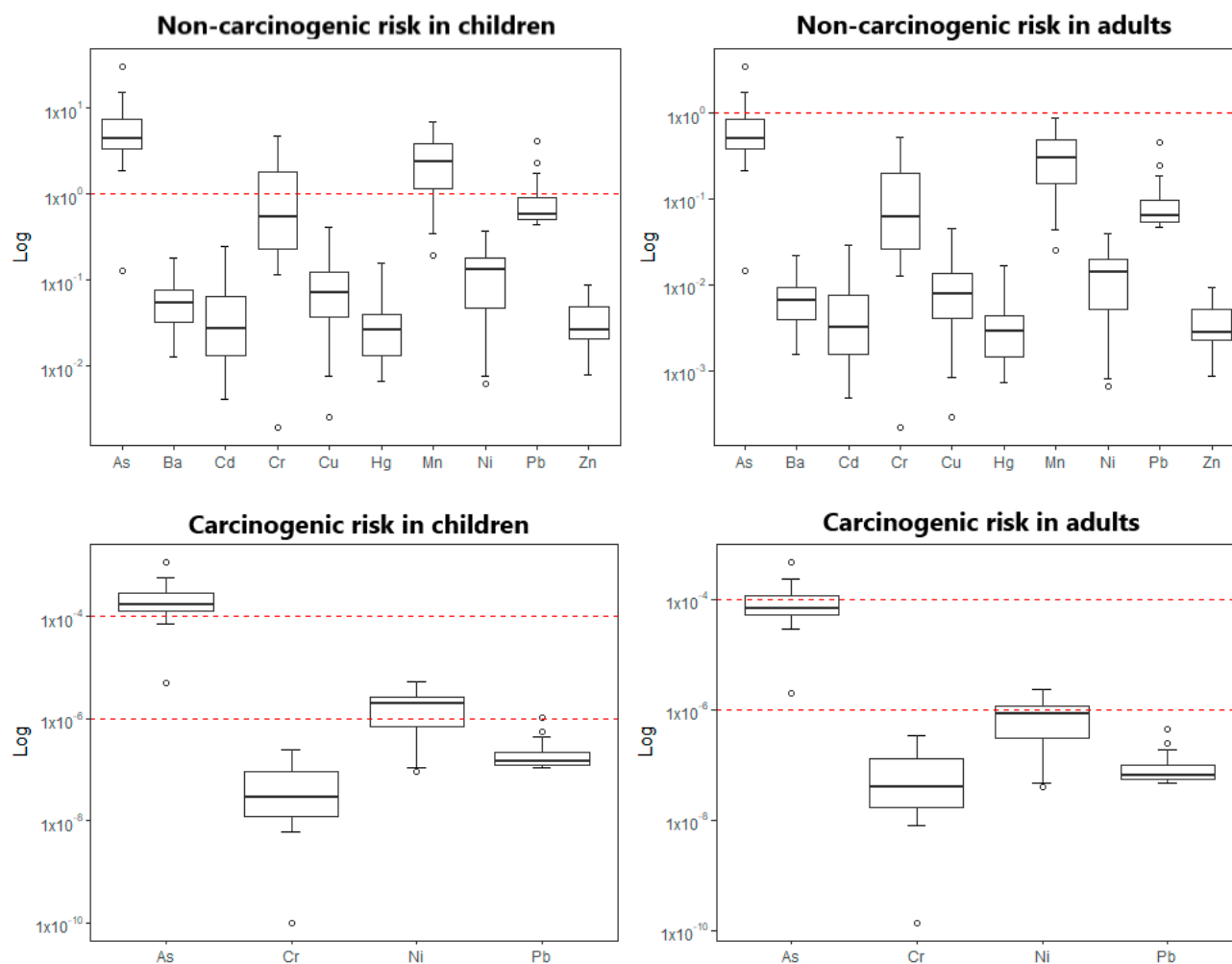
Figure 7. Box-plot diagrams for carcinogenic and non-carcinogenic risks in children and adults.
